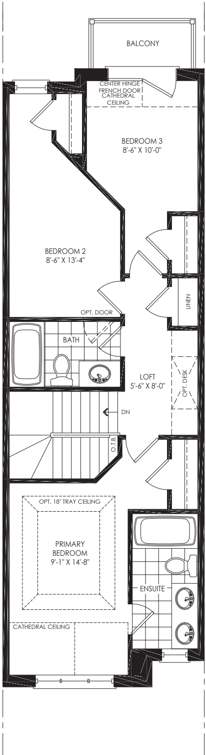
THIRD LEVEL ELEV A
