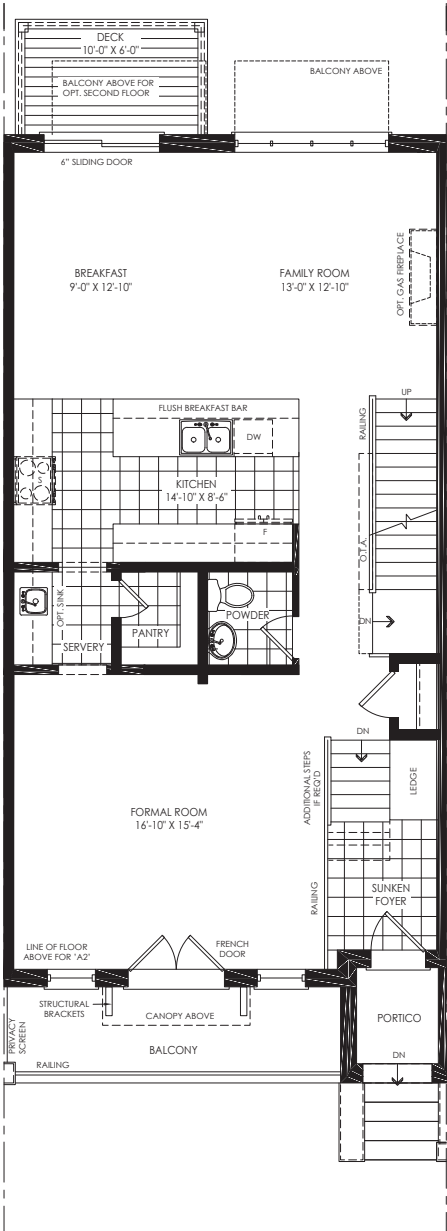
SECOND LEVEL ELEV A
